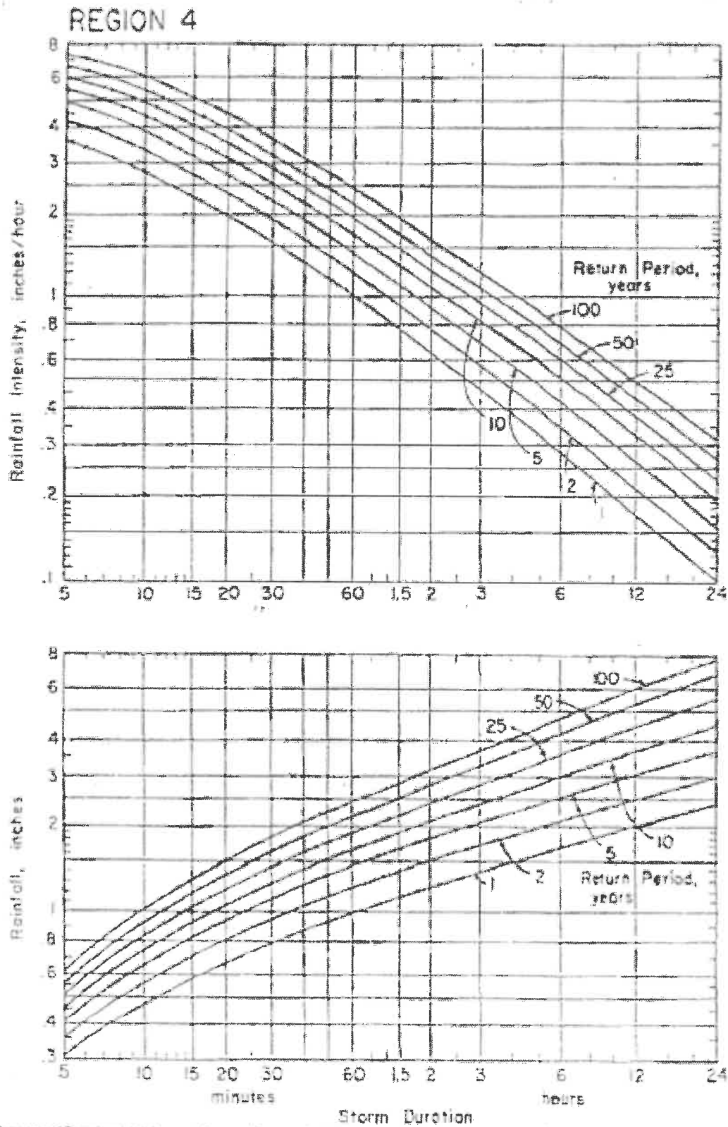
FIGURE B-3 PENNDOT REGION 4 STORM INTENSITY-DURATION-FREQUENCY CURVE
