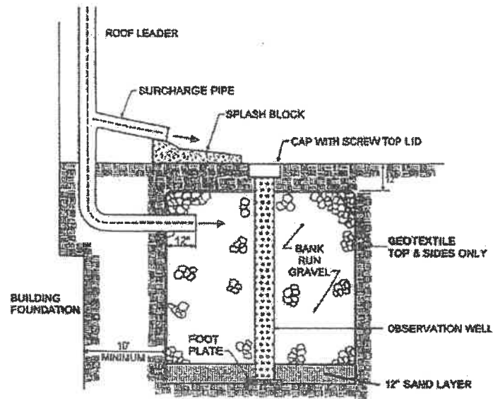
FIGURE I-1 TYPICAL DRY WELL CONFIGURATION
