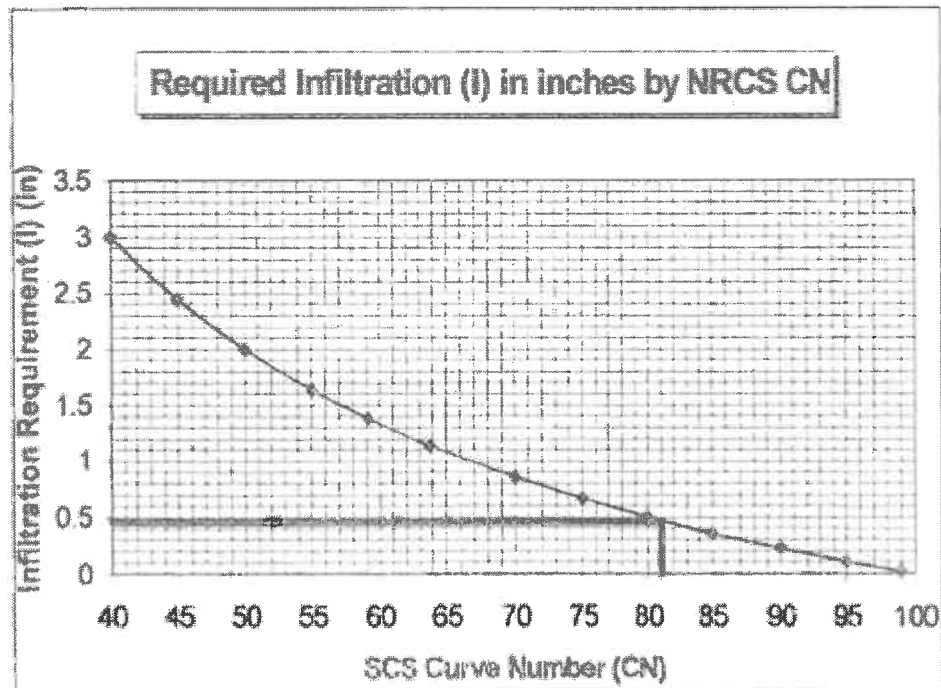
Figure 305.1. Infiltration requirement based upon NRCS Curve Number.
